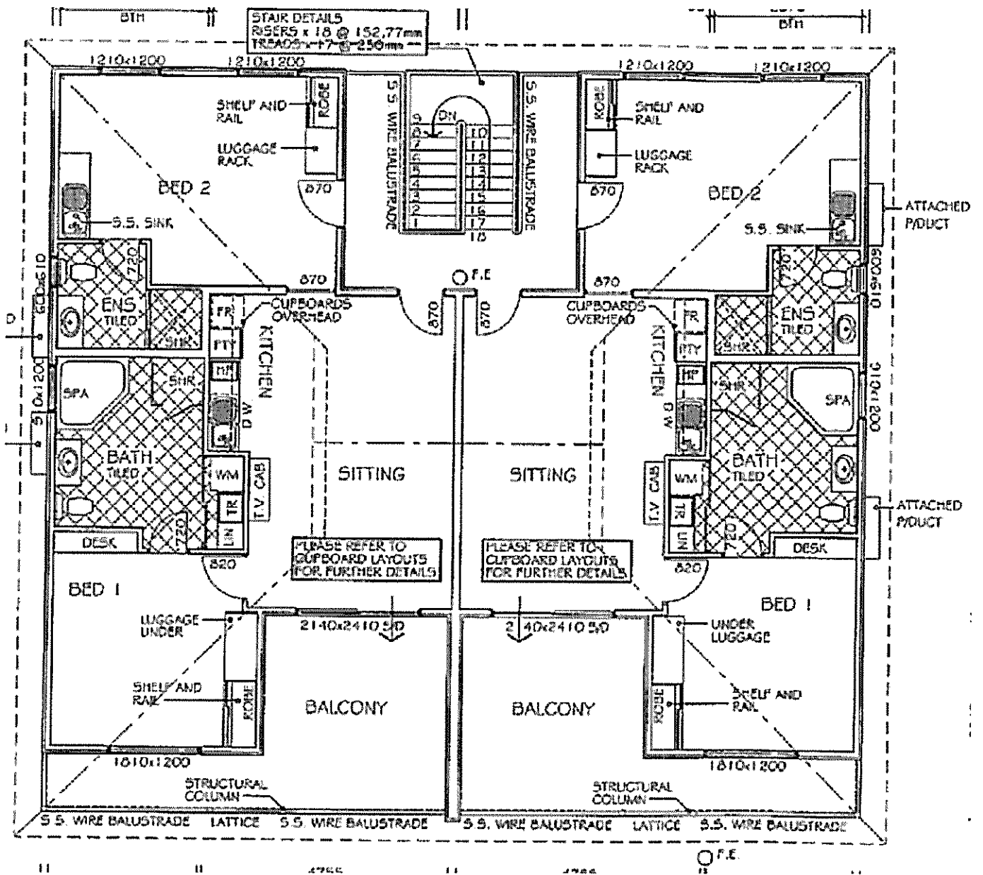
First Floor Typical Unit
